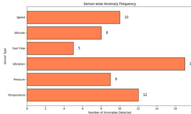
Fig 7. Anomaly Frequency
