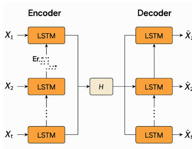
Fig. 2. Autoencoder-LSTM Architecture
