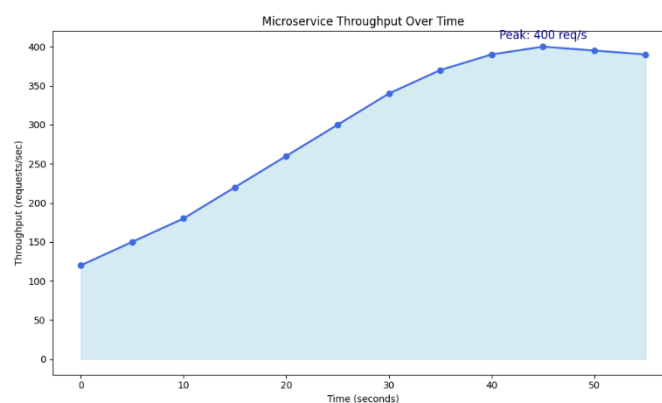
Fig 6. Throughput
