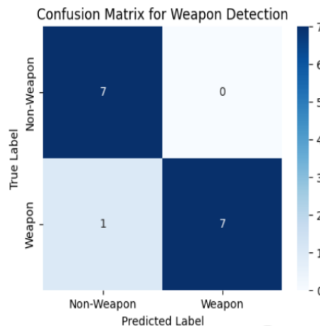
FIG 3. CONFUSION MATRIX
