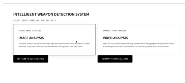
FIG 5. ANALYSIS PAGE
